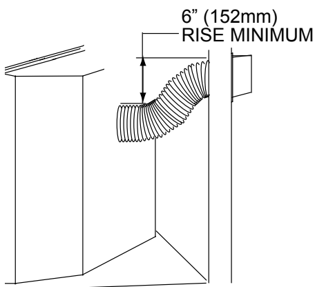
FLEXIBLE VENTING
