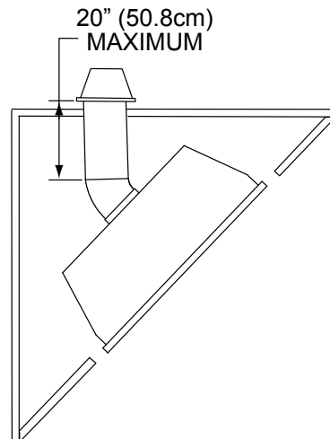
RIGID VENTING
